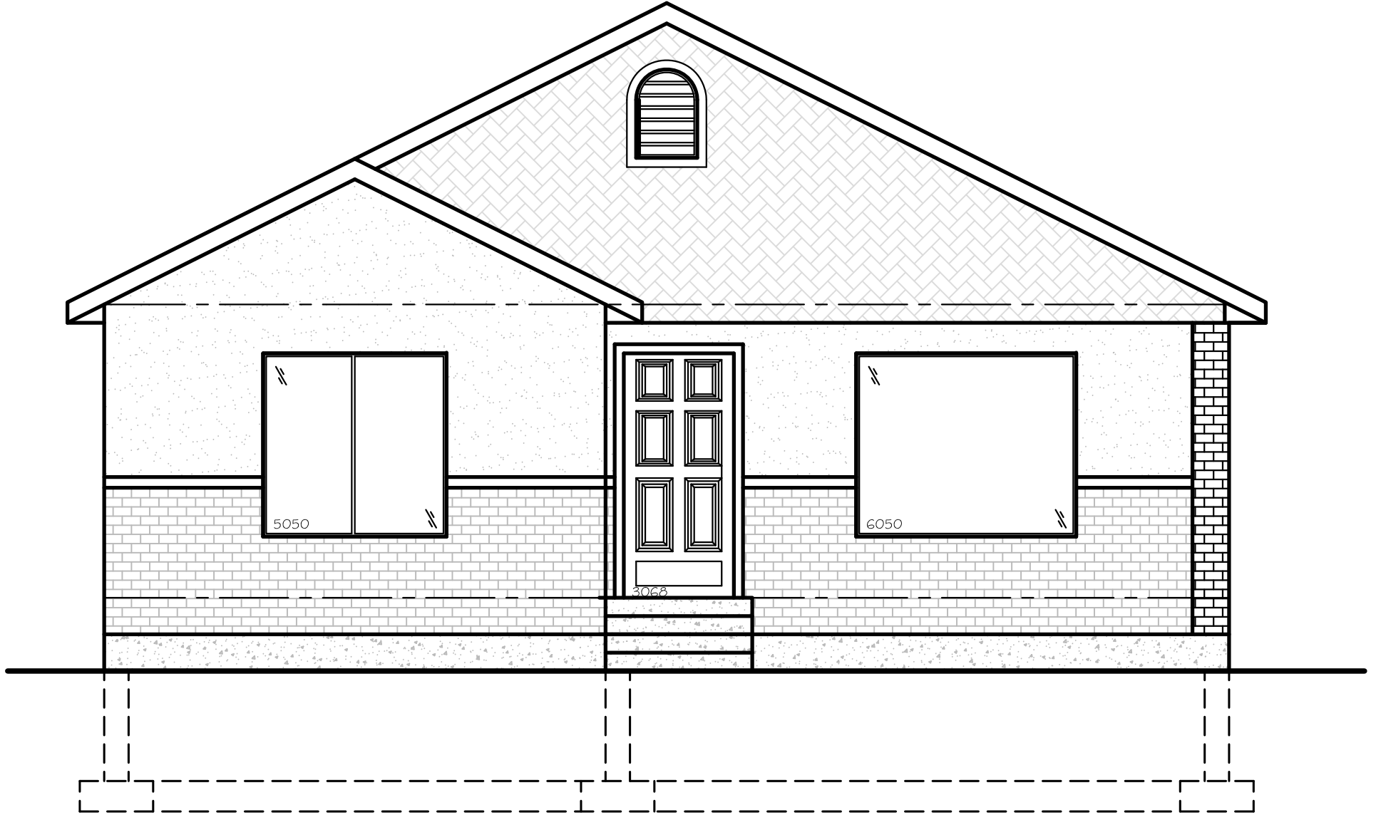
PRINT 5 FRONT ELEVATION
