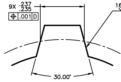
DETAIL A (5X)
