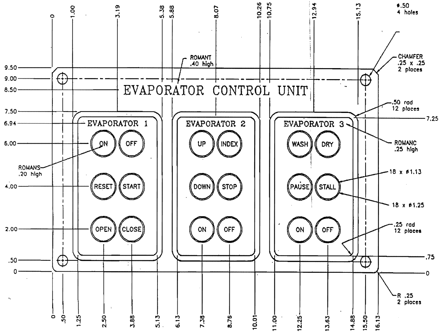
EVAPORATOR CONTROL UNIT
